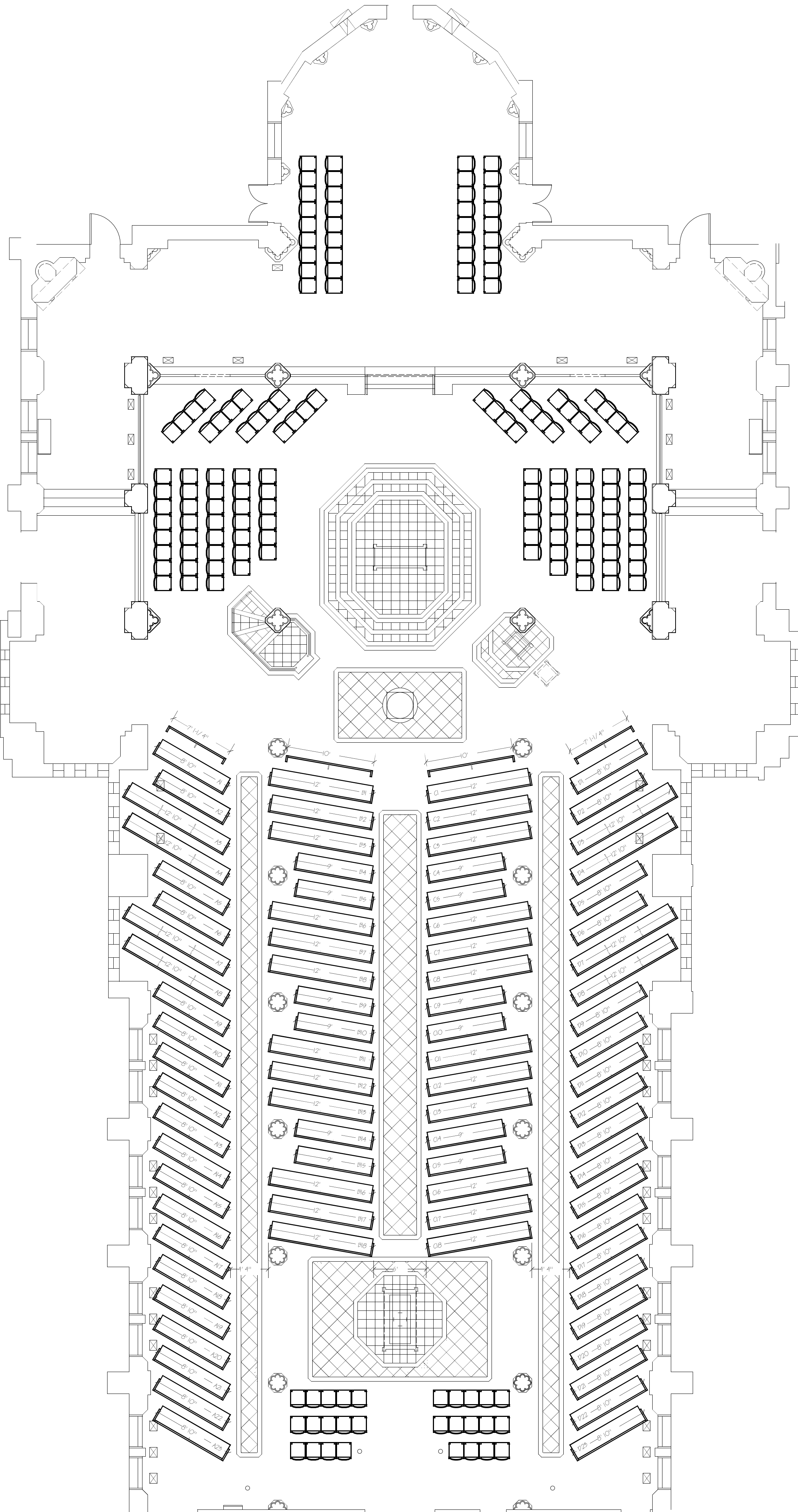
SEATING LAYOUT SCALE: 1/8"=1'
